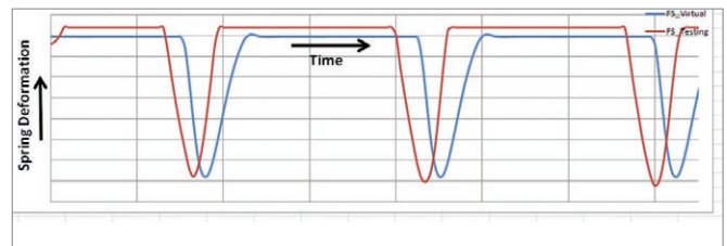
Correlation between MBD simulation and testing on front suspension
