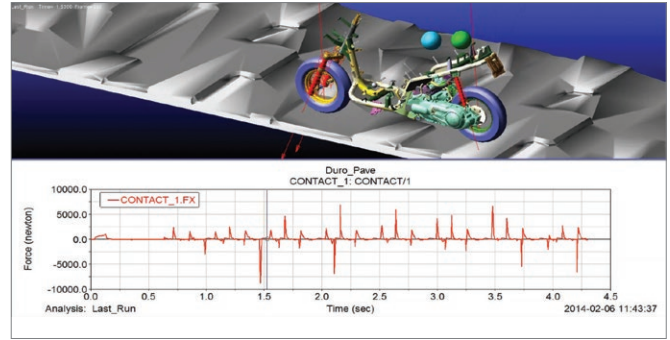
Rough road riding test using Adams
