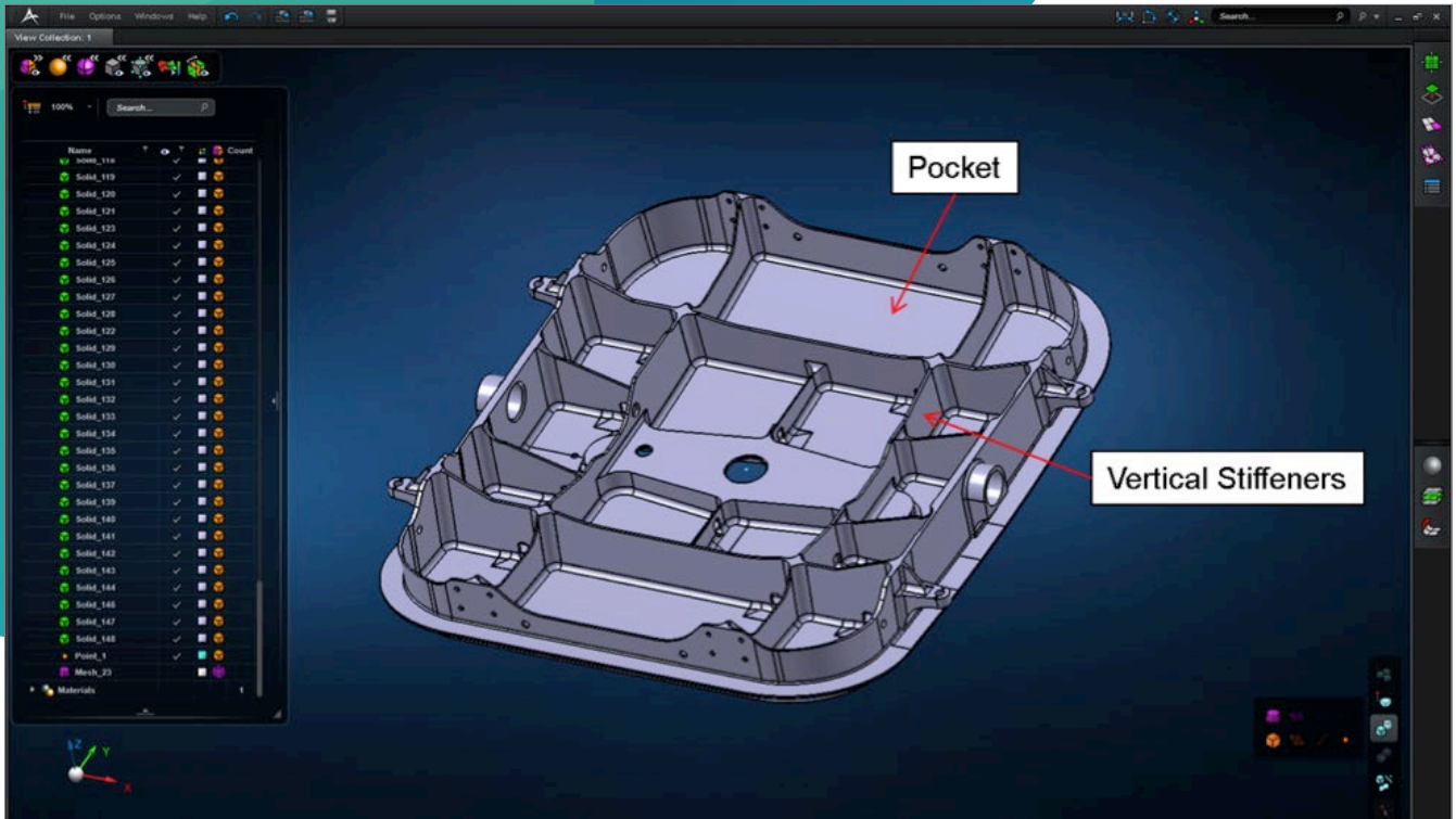
Fig. 1: CAD model inside MSC Apex
