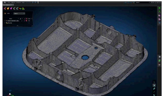
Fig. 3: Finite element mesh inside MSC Apex
