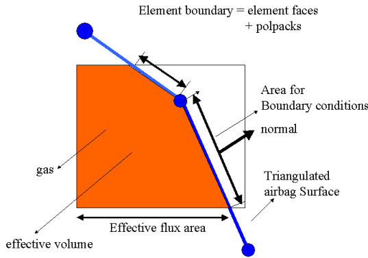
Figure 1: The boundary of an element
