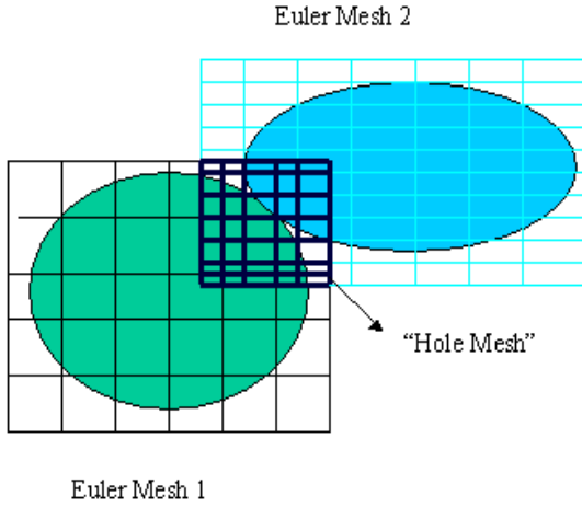
Figure 2: Assembling the hole mesh
