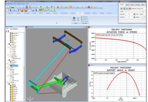
Railway pantograph
